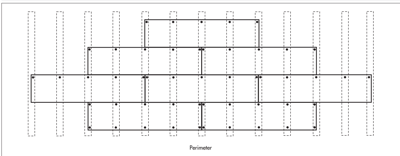
Figure 2 Nailing pattern for 2400 mm x 600 mm boards fixed to I-joists at 600 mm centres
